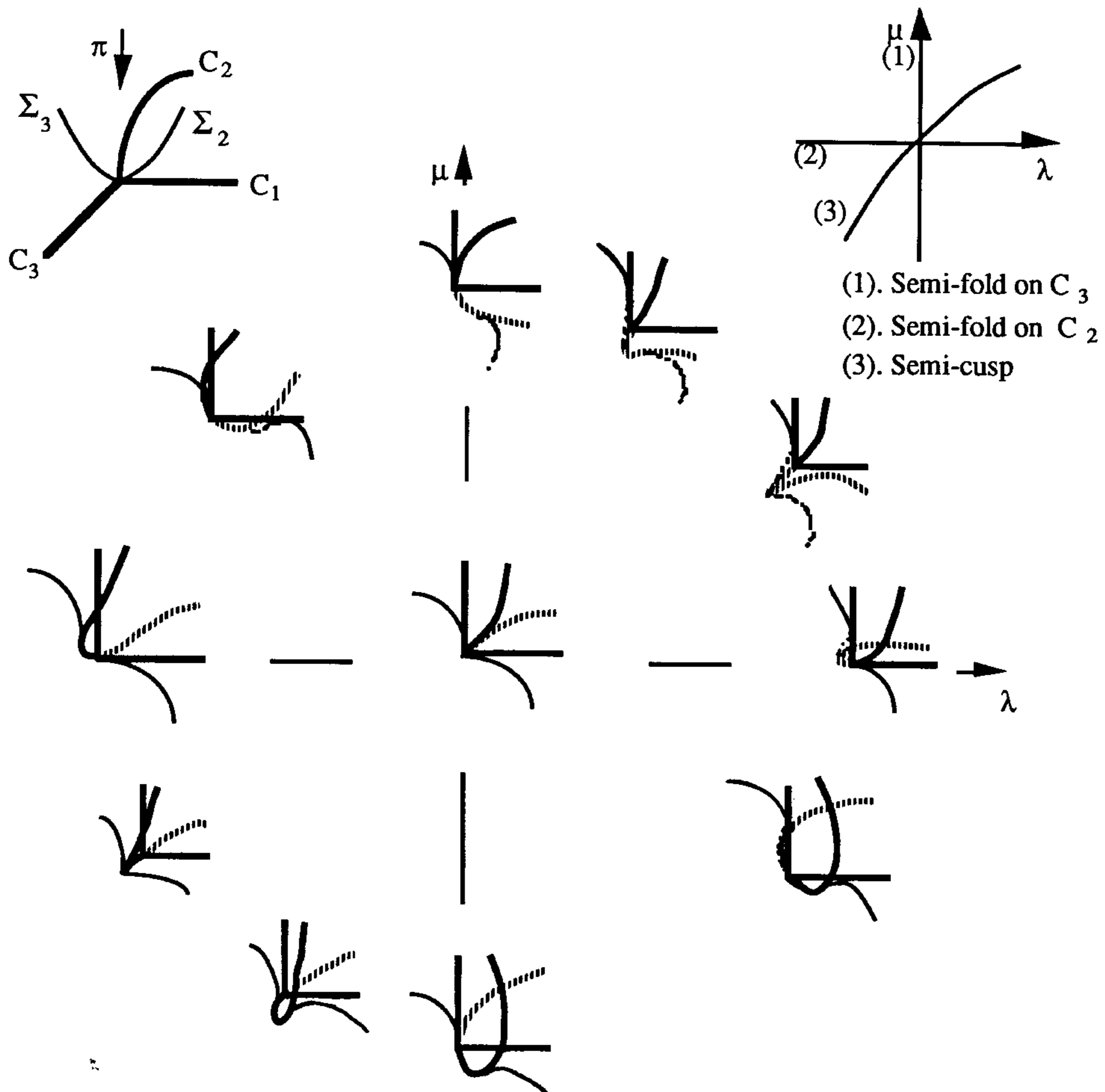
Figure 2.4.4. C-crease-cusp
