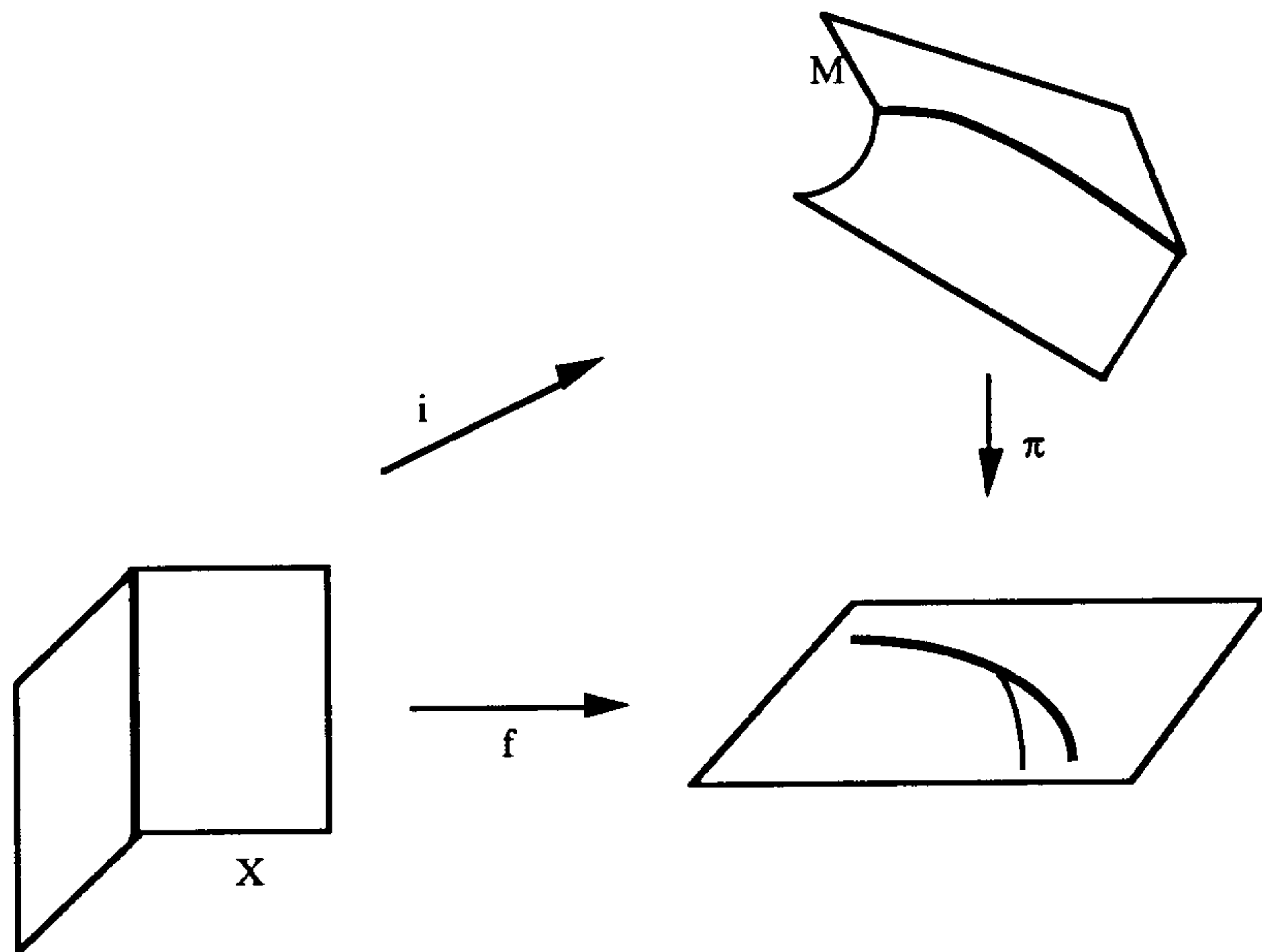
Figure 1.1.1. Projection of a piecewise smooth surface
