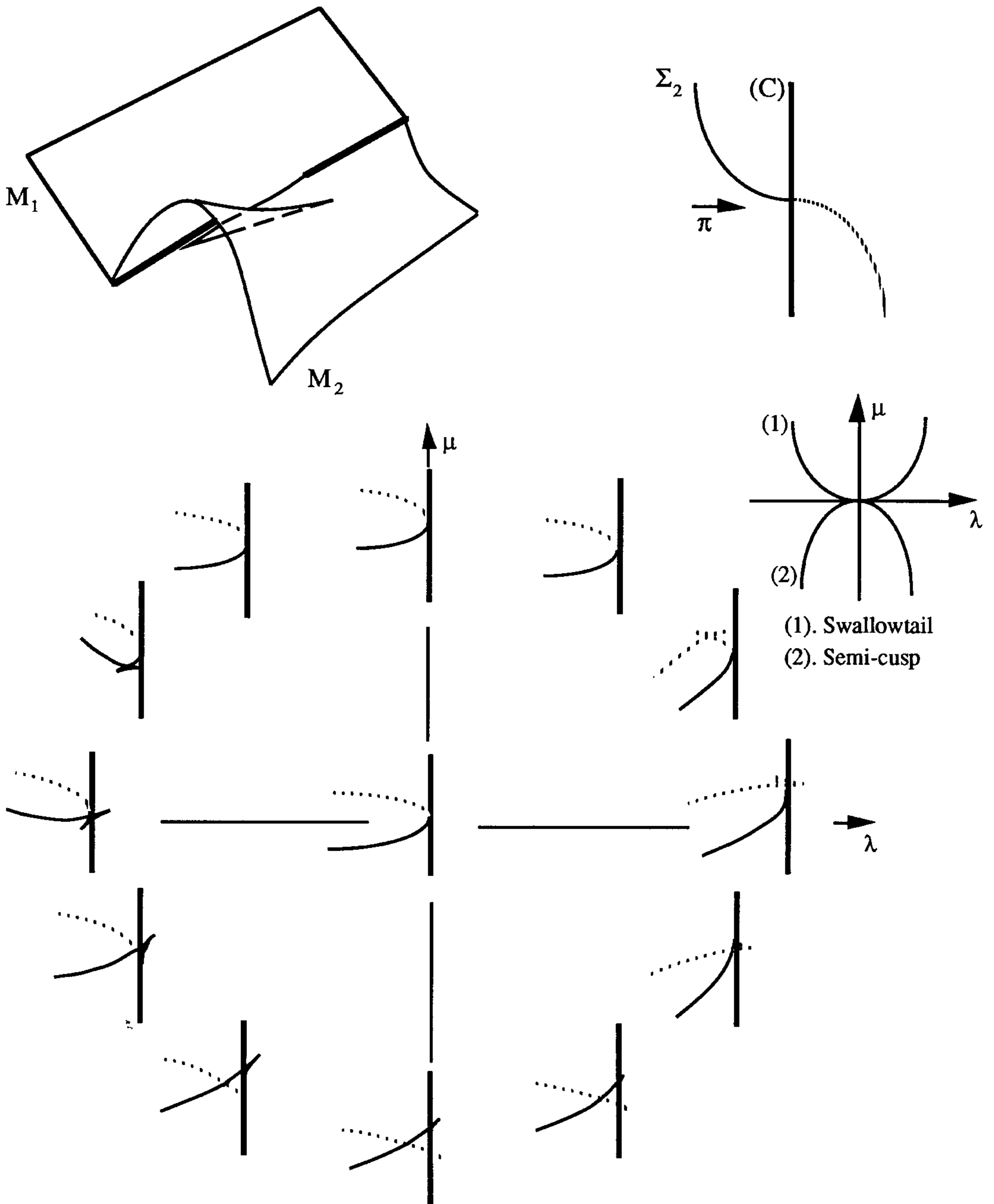
Figure 1.4.5. Semi-swallowtail
