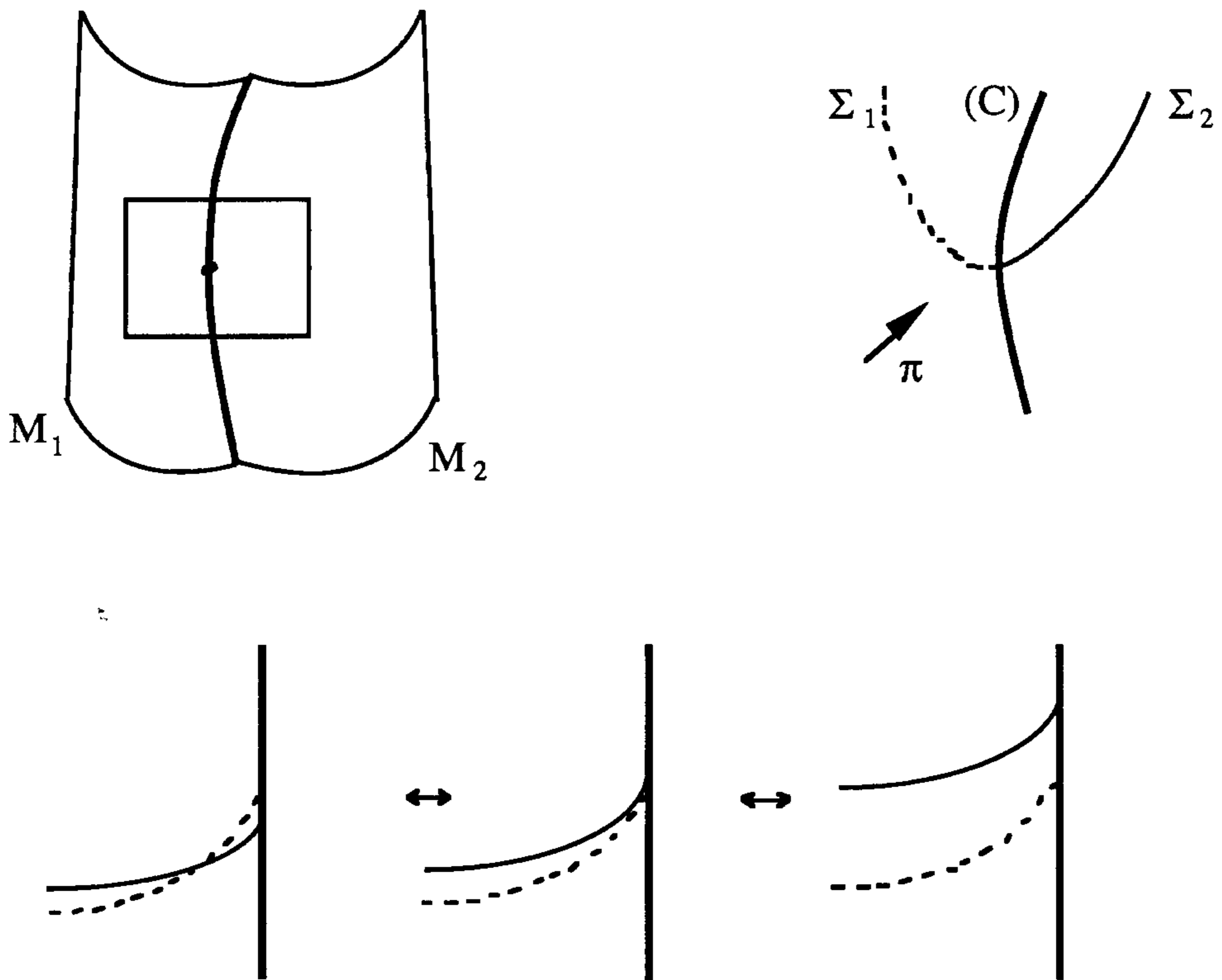
Figure 1.4.10. Non-transverse semi-fold
