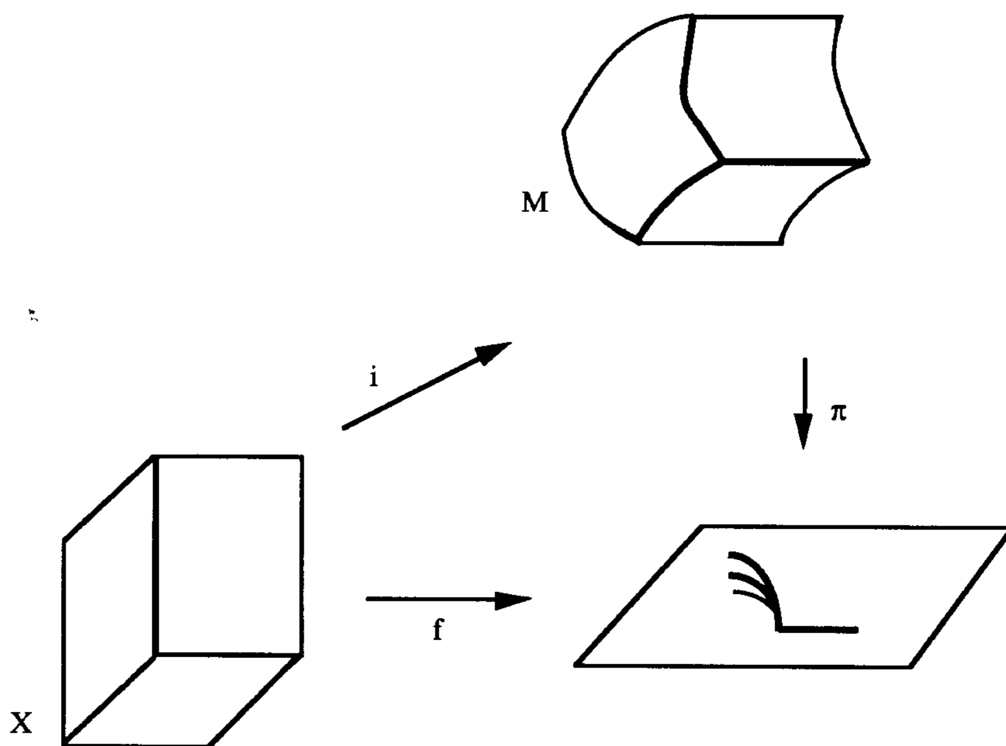
Figure 2.1.1. Projection of a triple of surfaces
