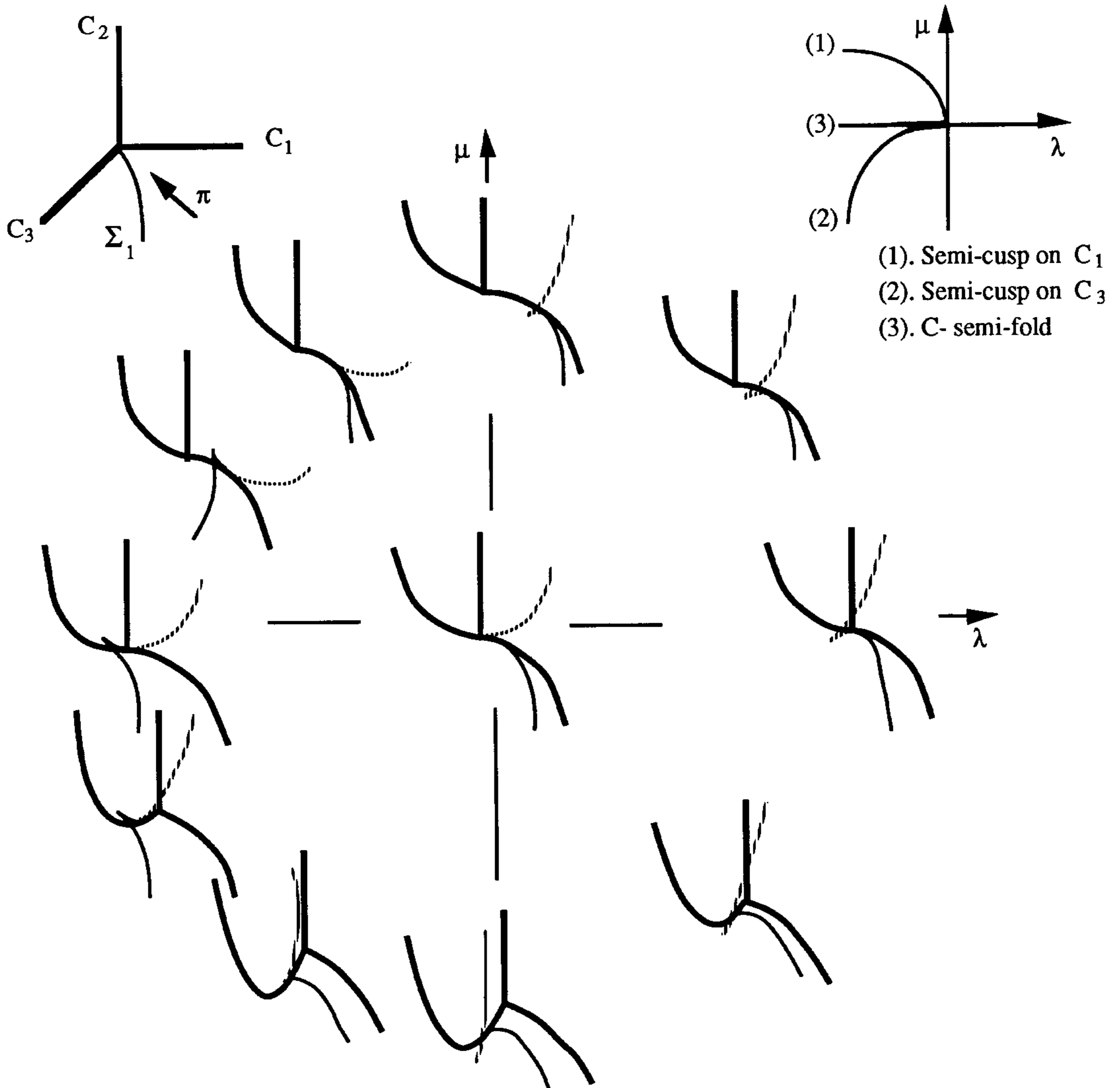
Figure 2.4.2. C- Semi-cusp
