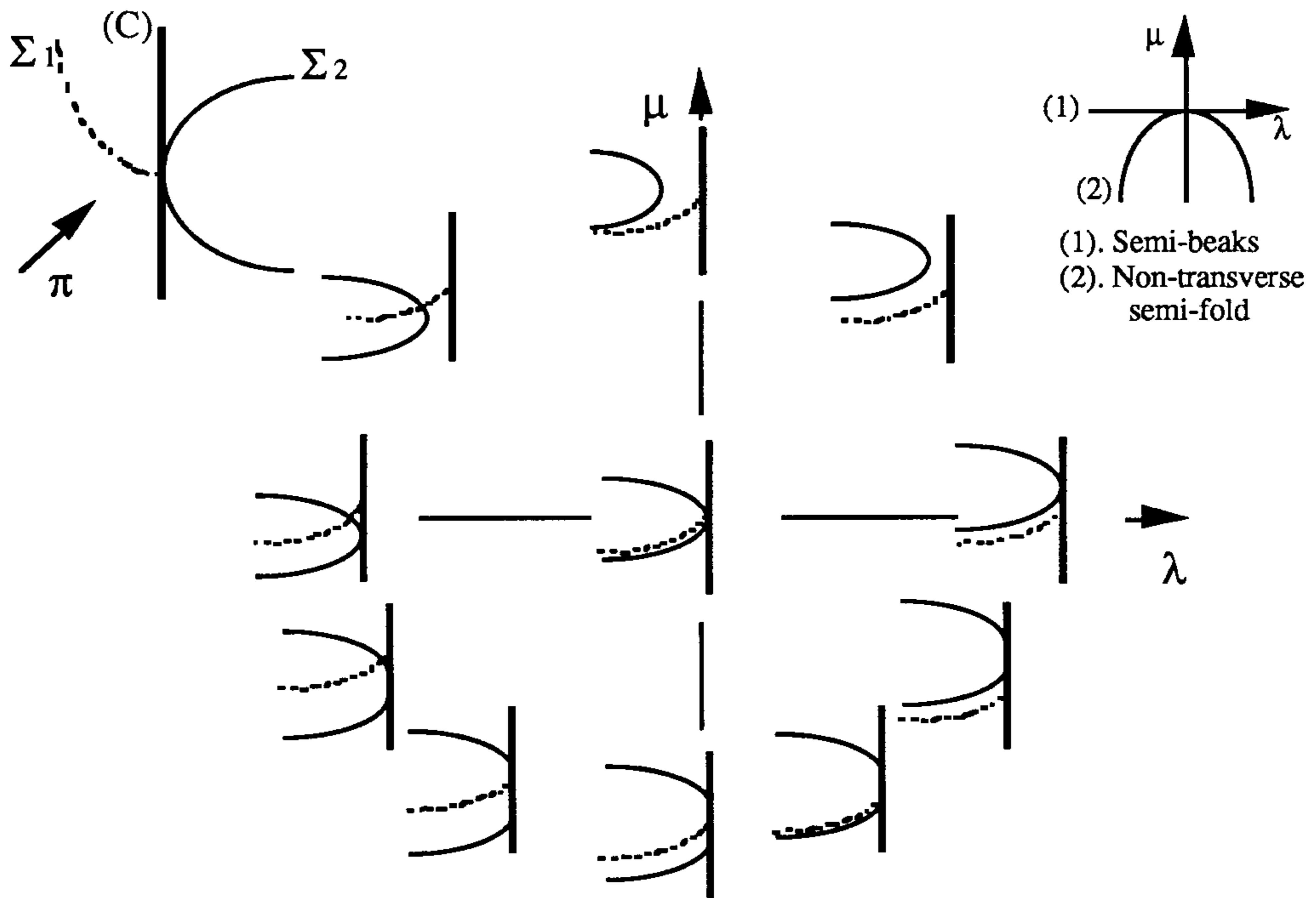
Figure 1.4.12. Non-transverse semi-beaks
