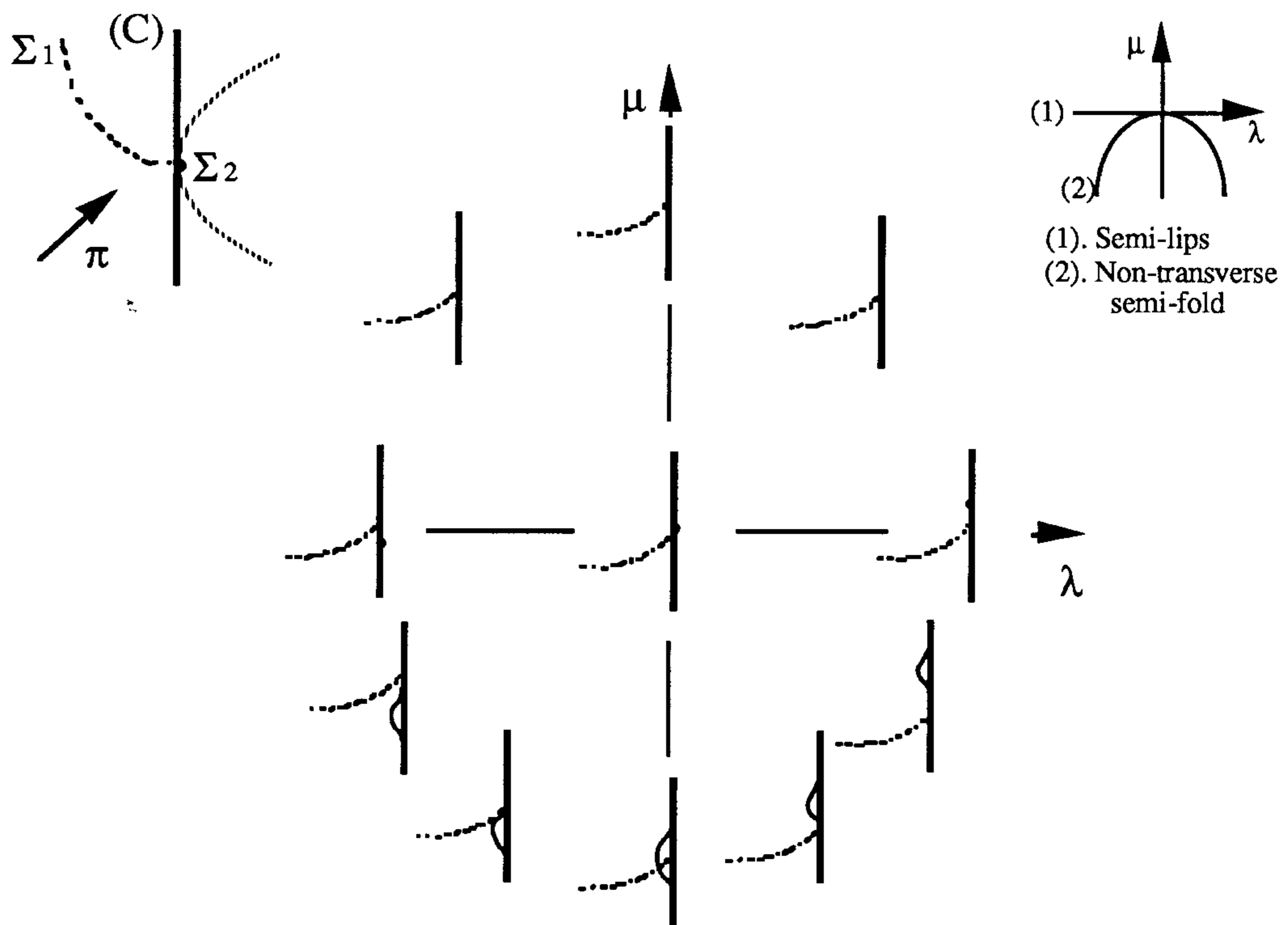
Figure 1.4.11. Non-transverse semi-lips
