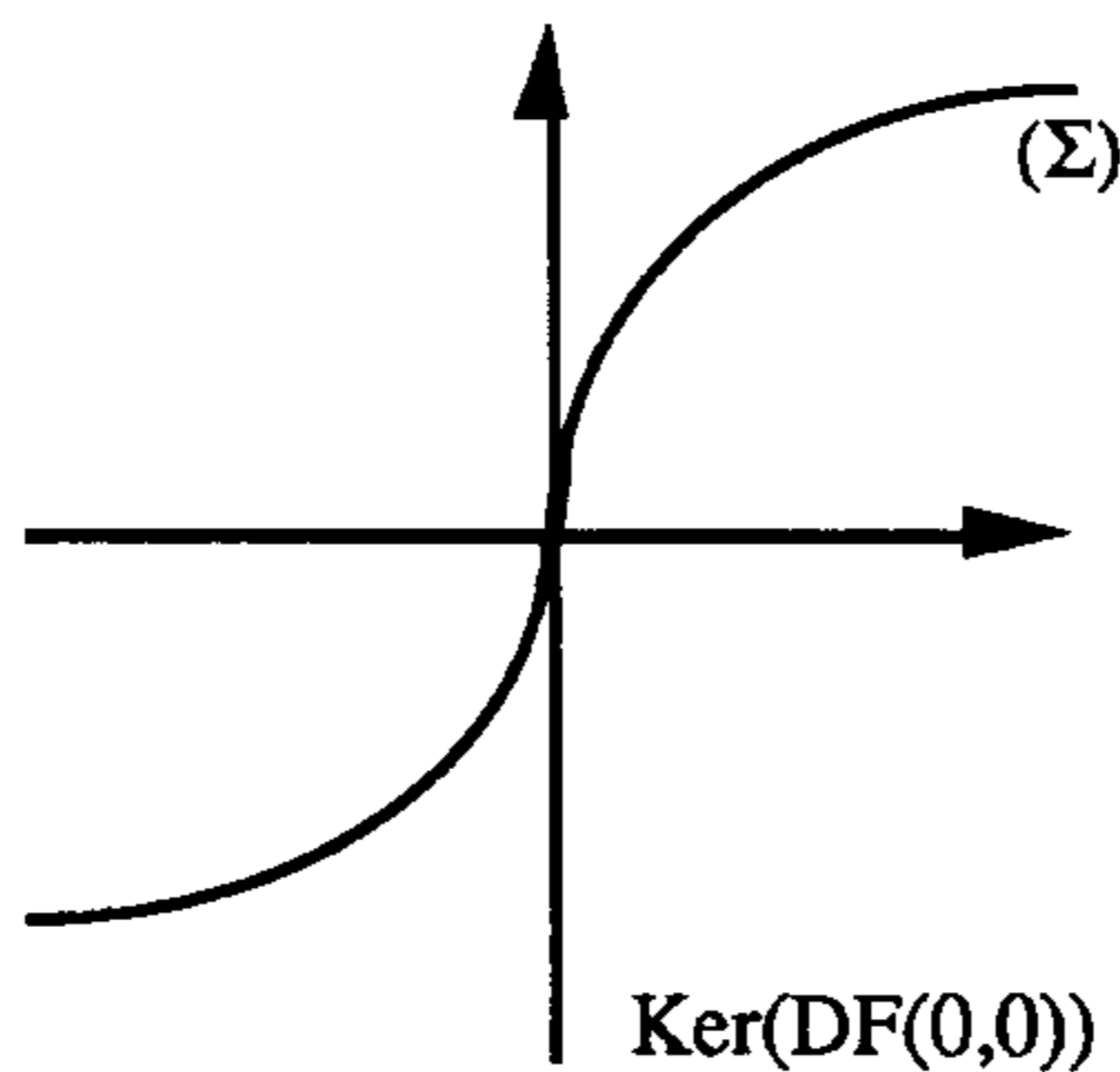
Figure 3.3.1 A swallowtail map
