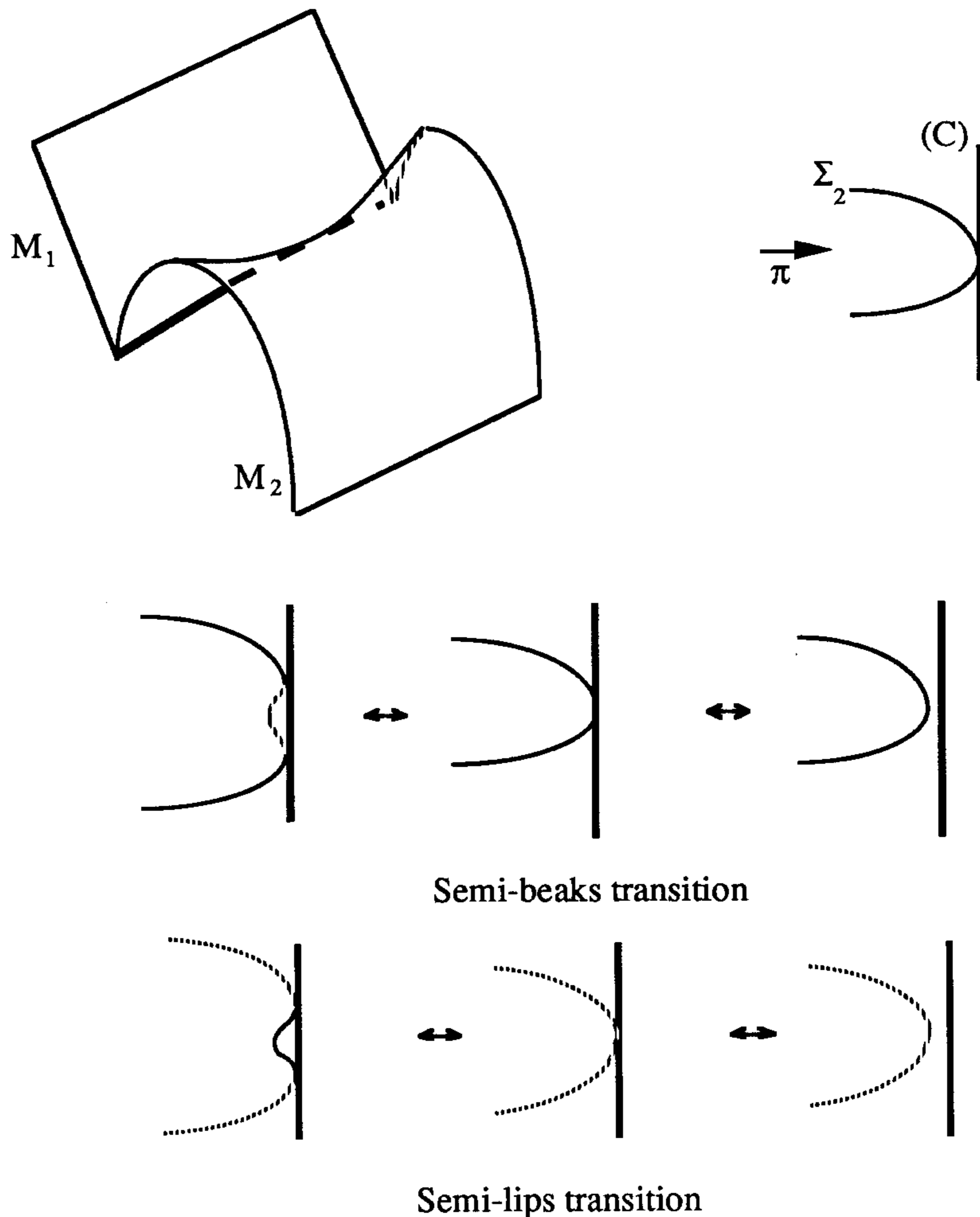
Figure 1.4.2. Semi-lips/beaks
