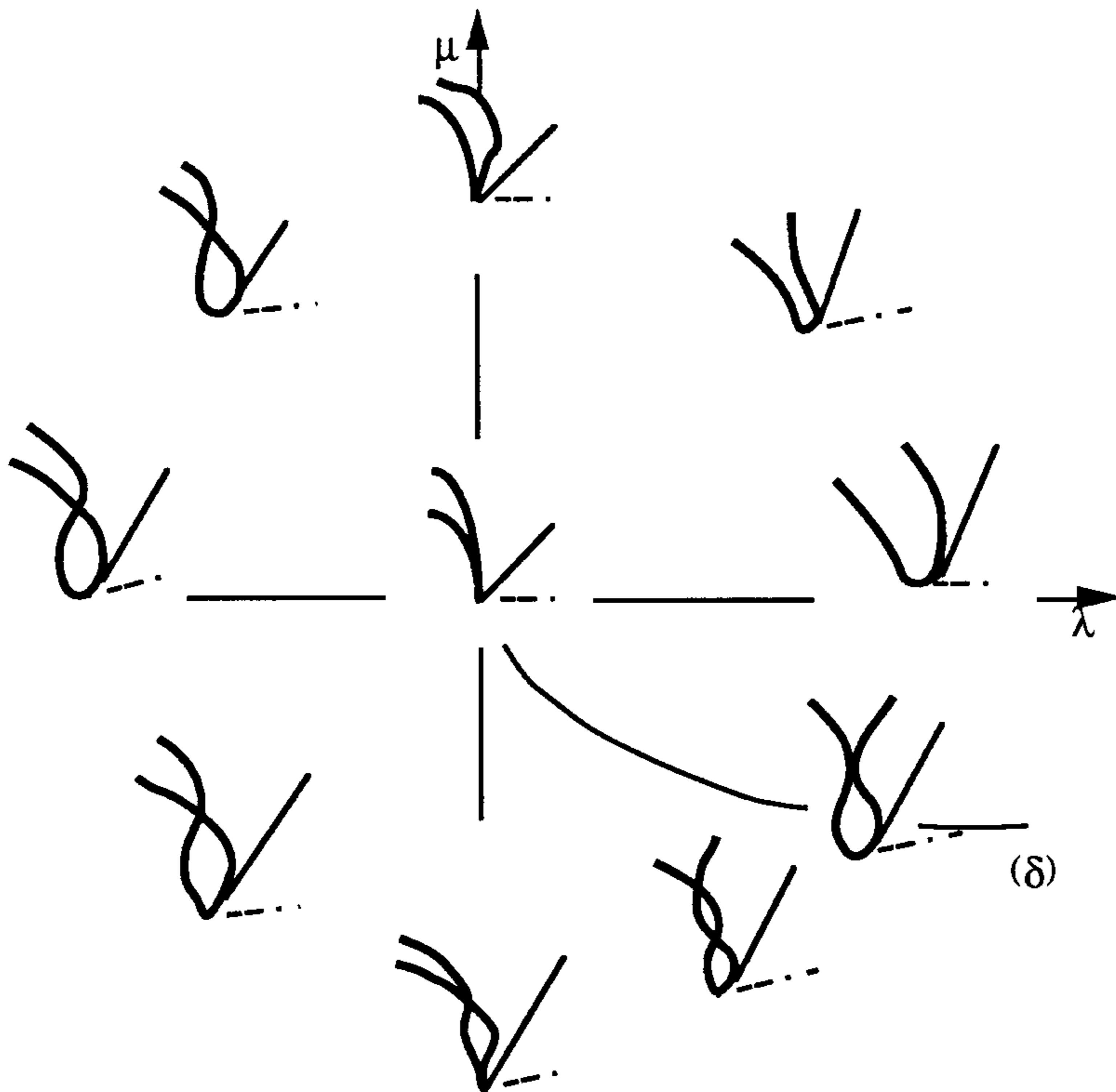
Figure 1.4.8. Crease rhamphoid cusp
