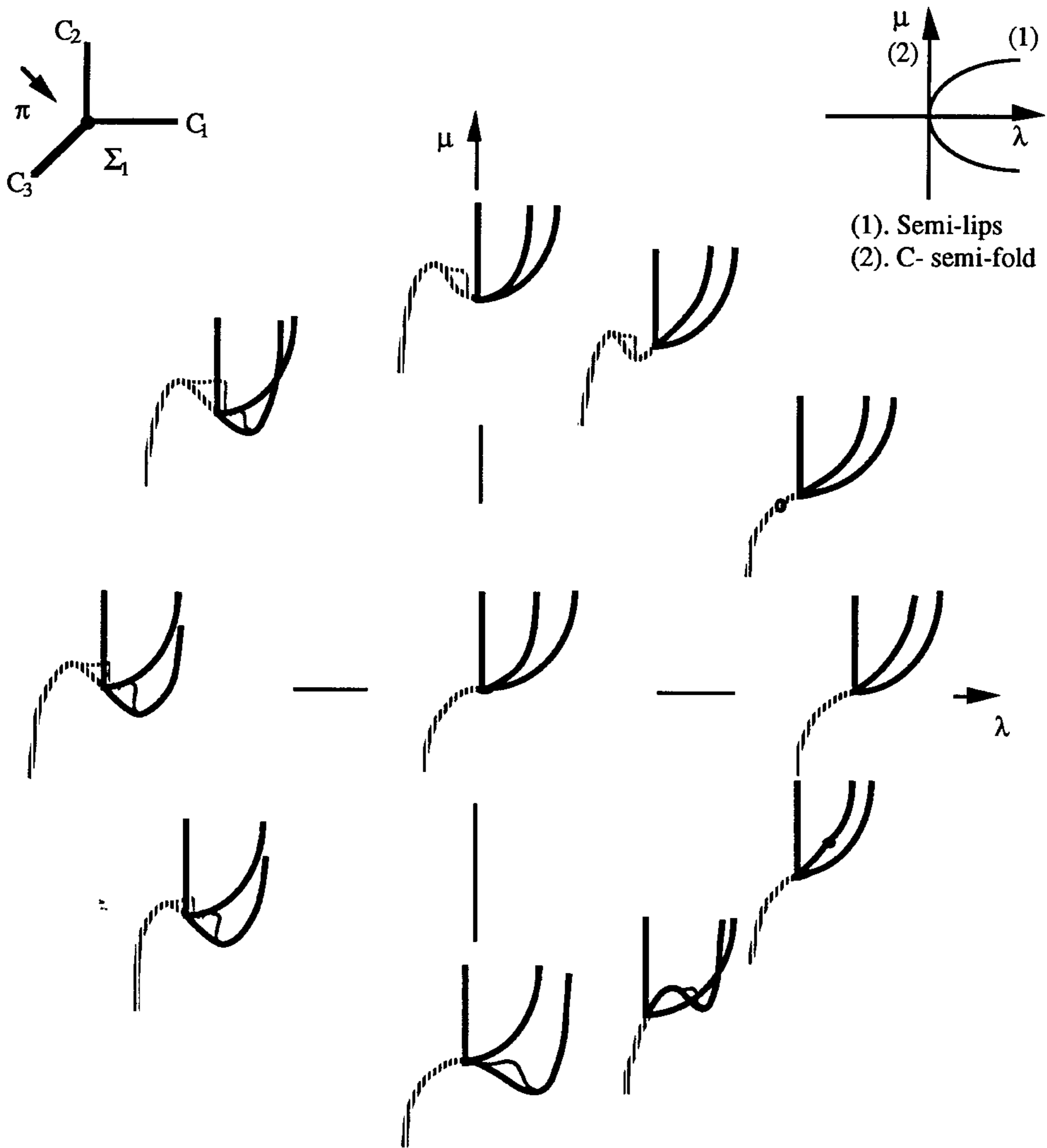
Figure 2.4.3. C- Semi-lips
