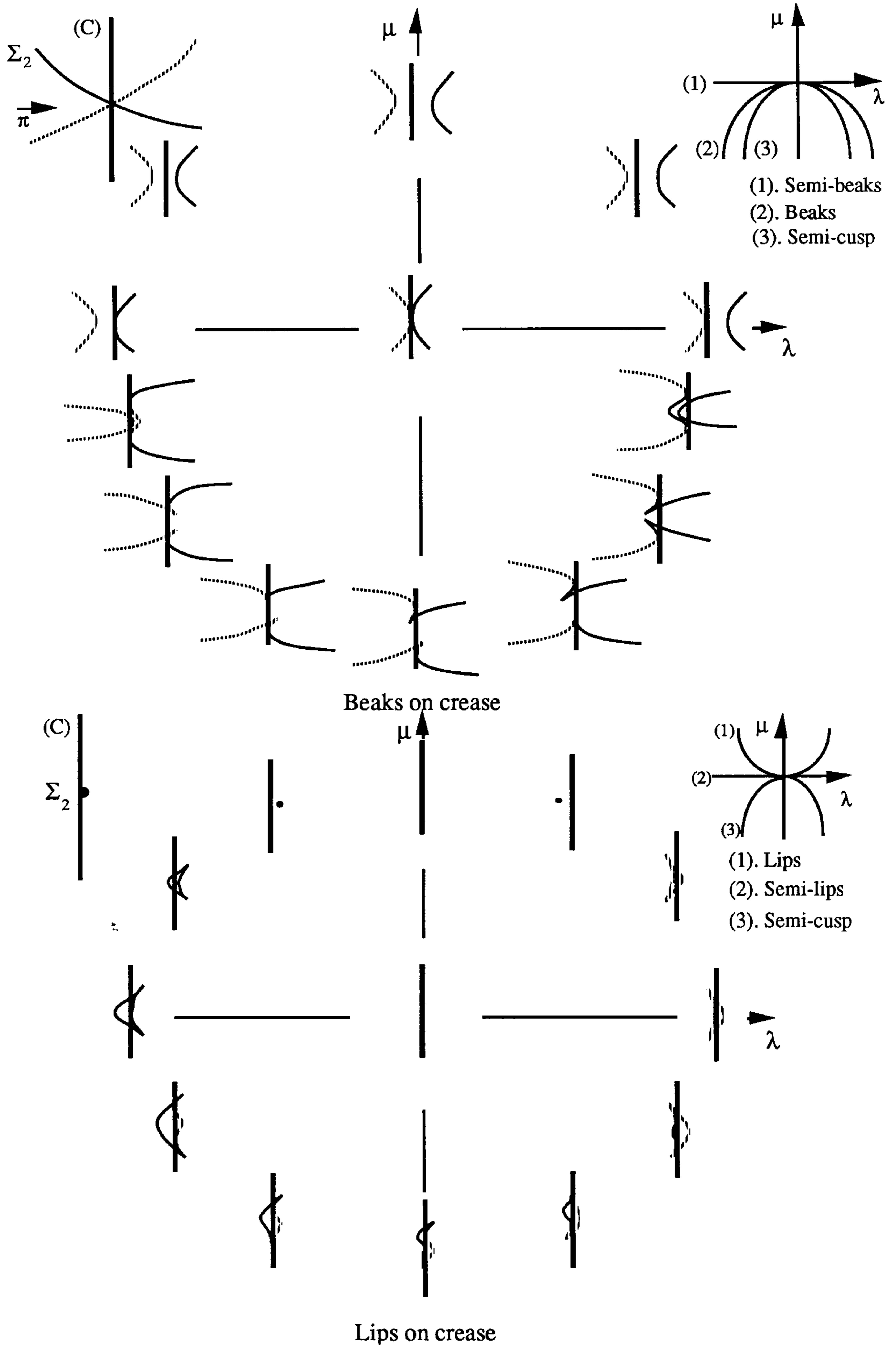
Figure 1.4.6. Lips/beaks on crease
