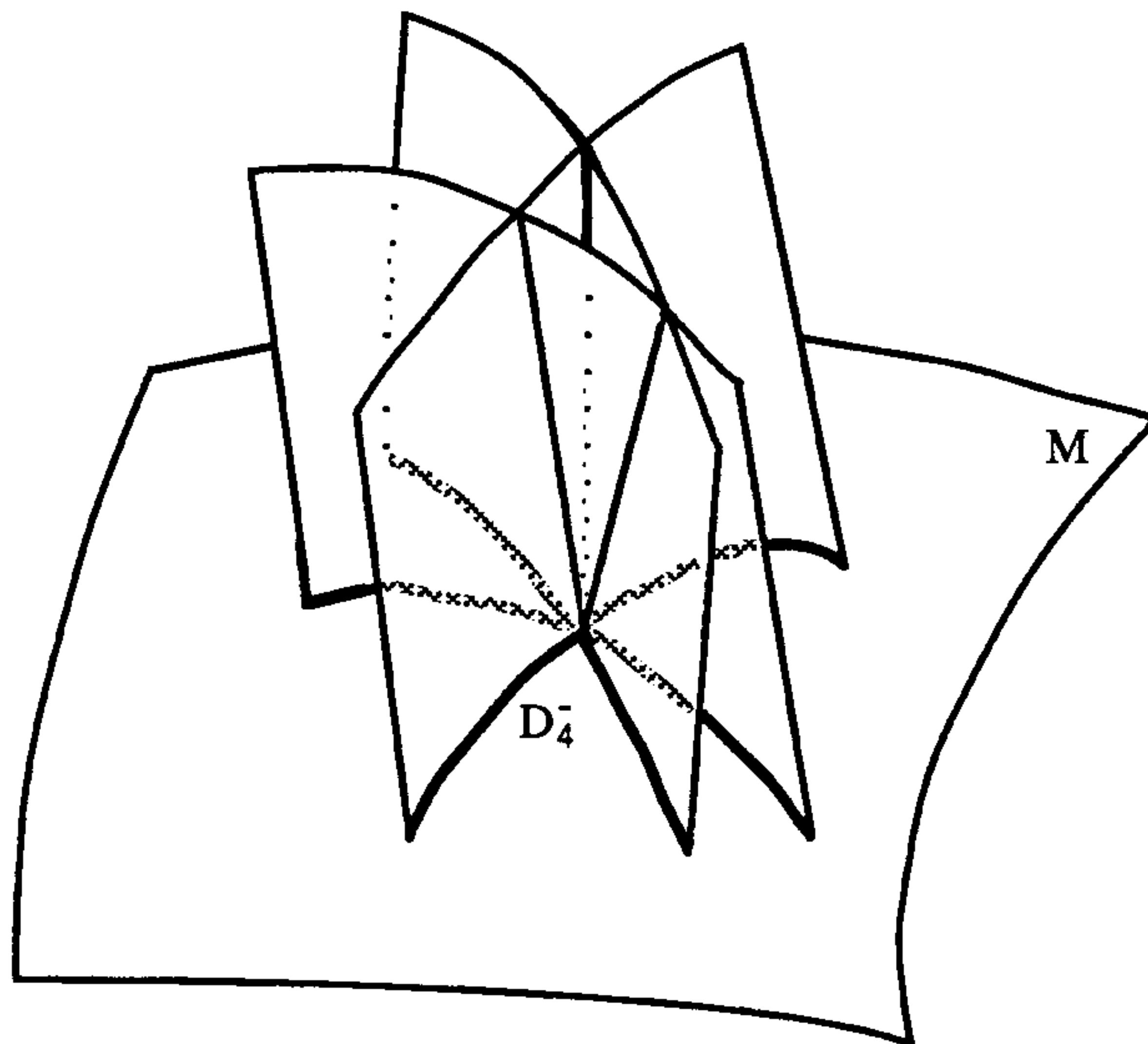
Figure 6.3.1. The midpoint locus at a D_4^- point
