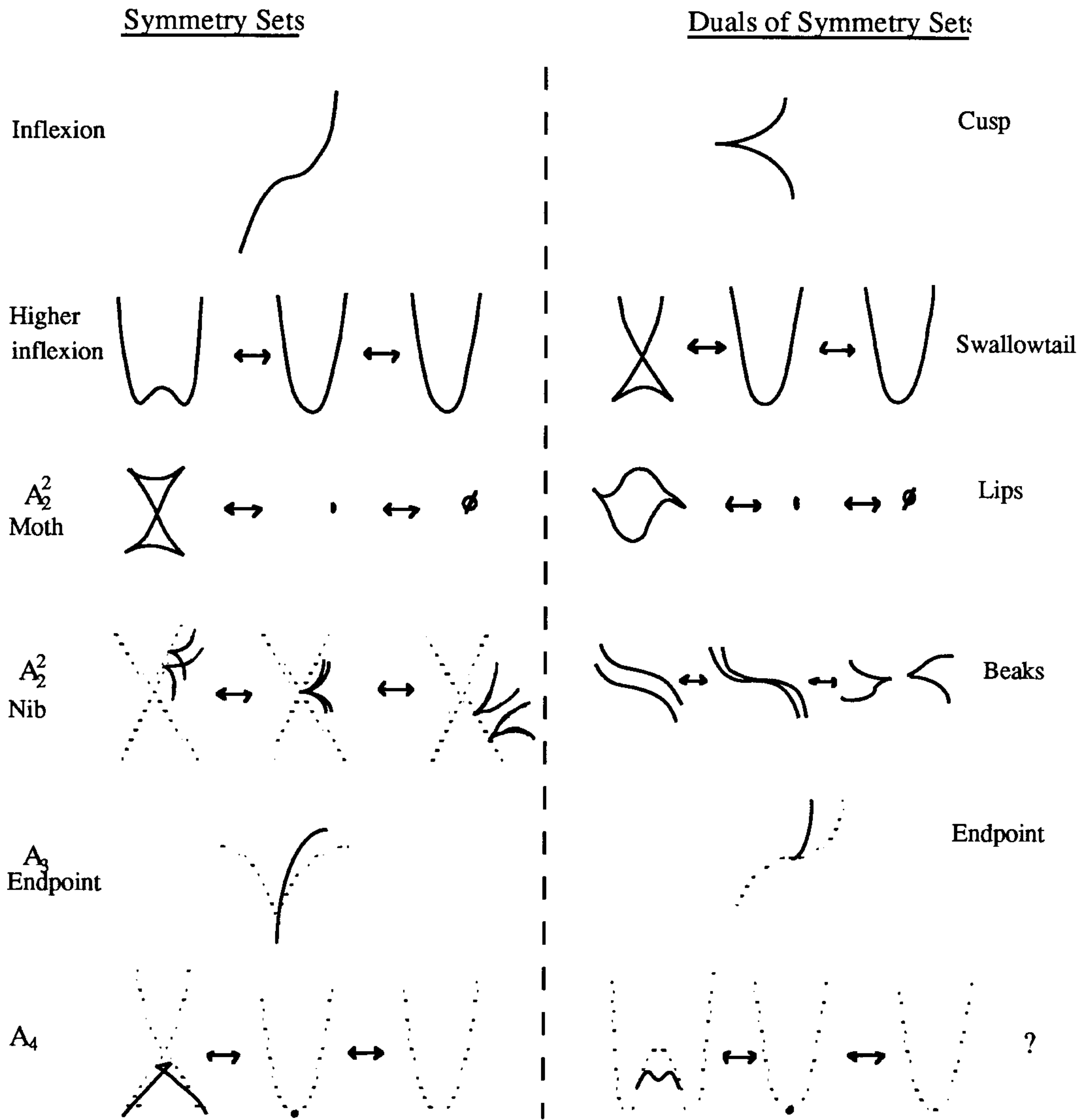
Figure 4.2.9. Transitions on 1-parameter families of duals of symmetry sets
