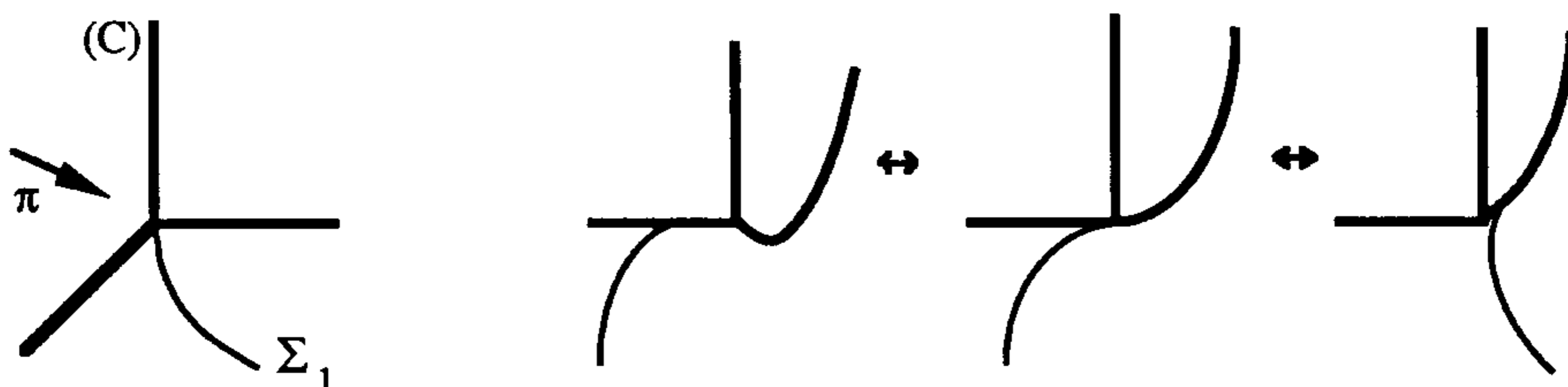
Figure 2.4.1. C- Semi-fold
