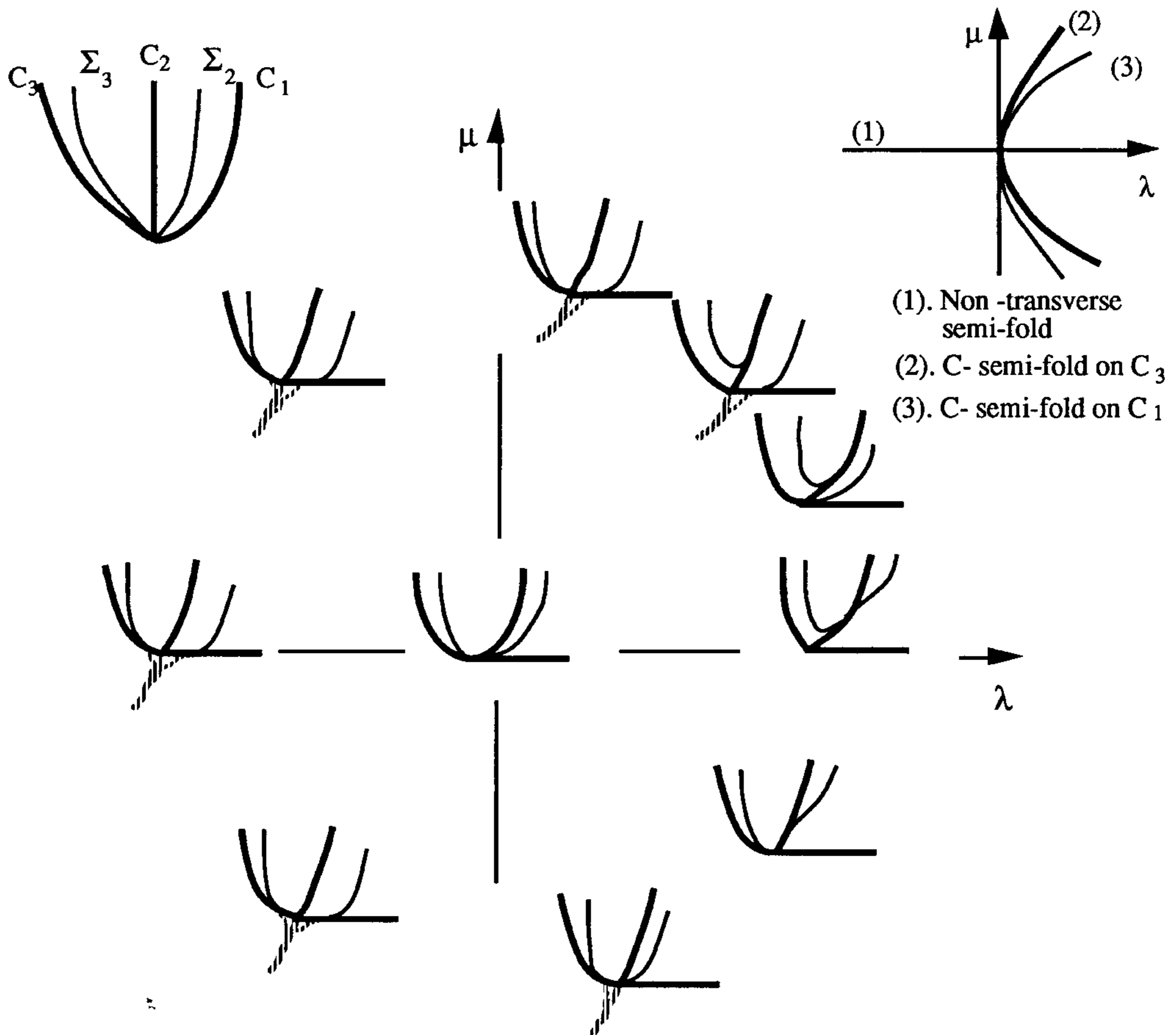
Figure 2.4.5. Non-transverse C- semi-fold
