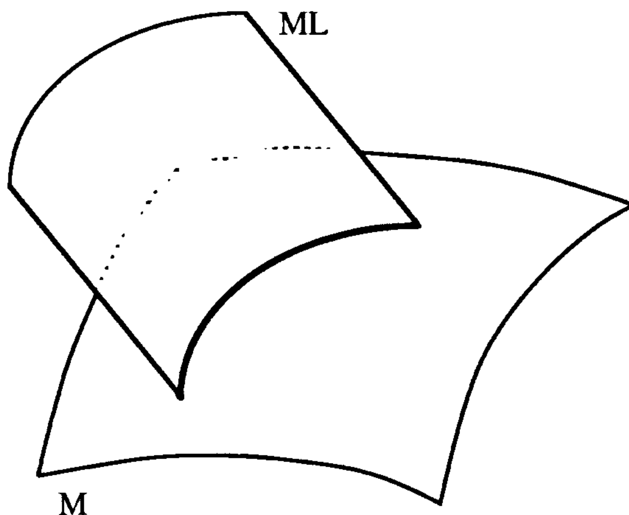
Figure 6.3.2. The midpoint locus at an A_3 point
