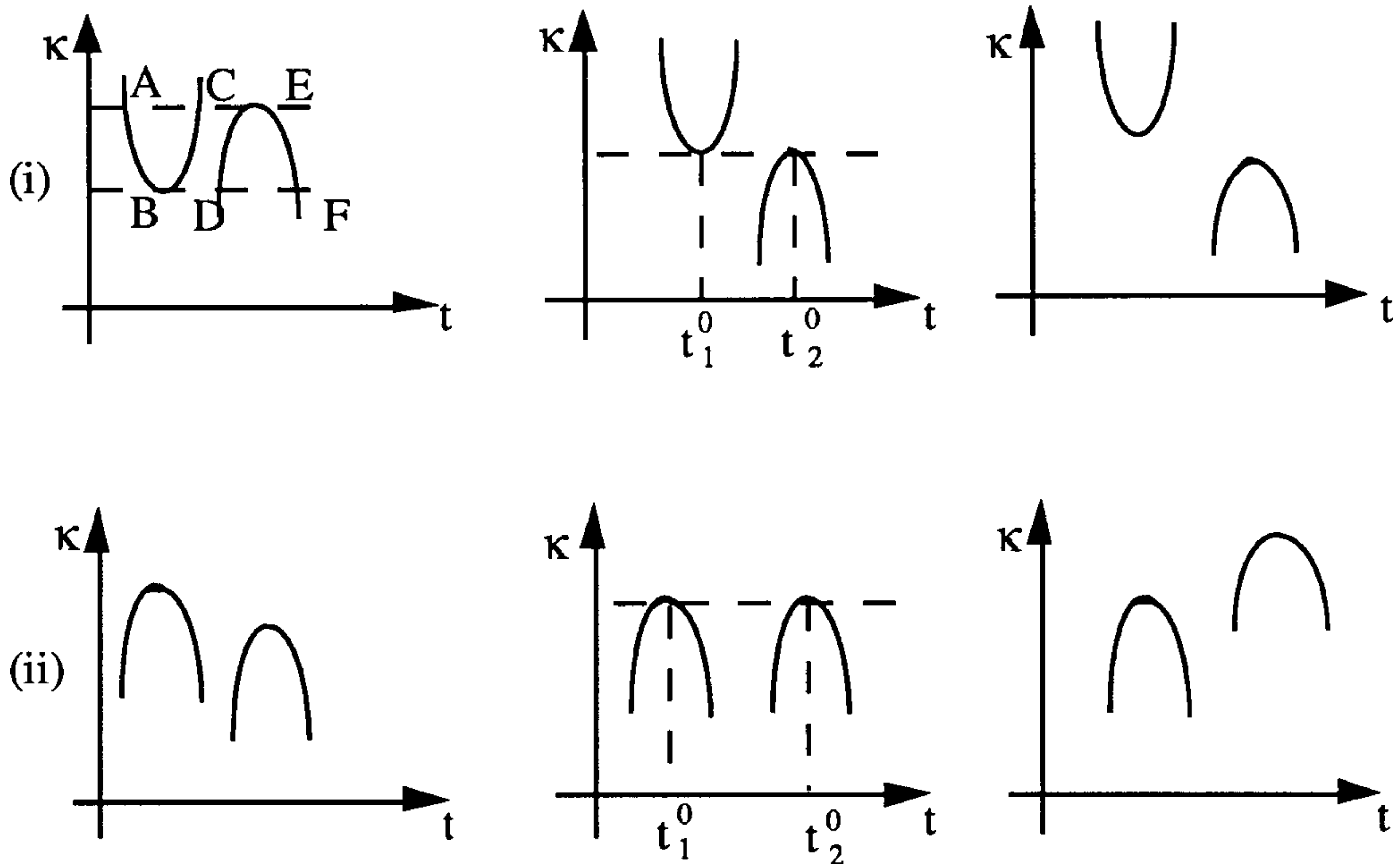
Figure 5.3.2. Changes in the \kappa -curve which give lips/beaks transitions on RSS^+
