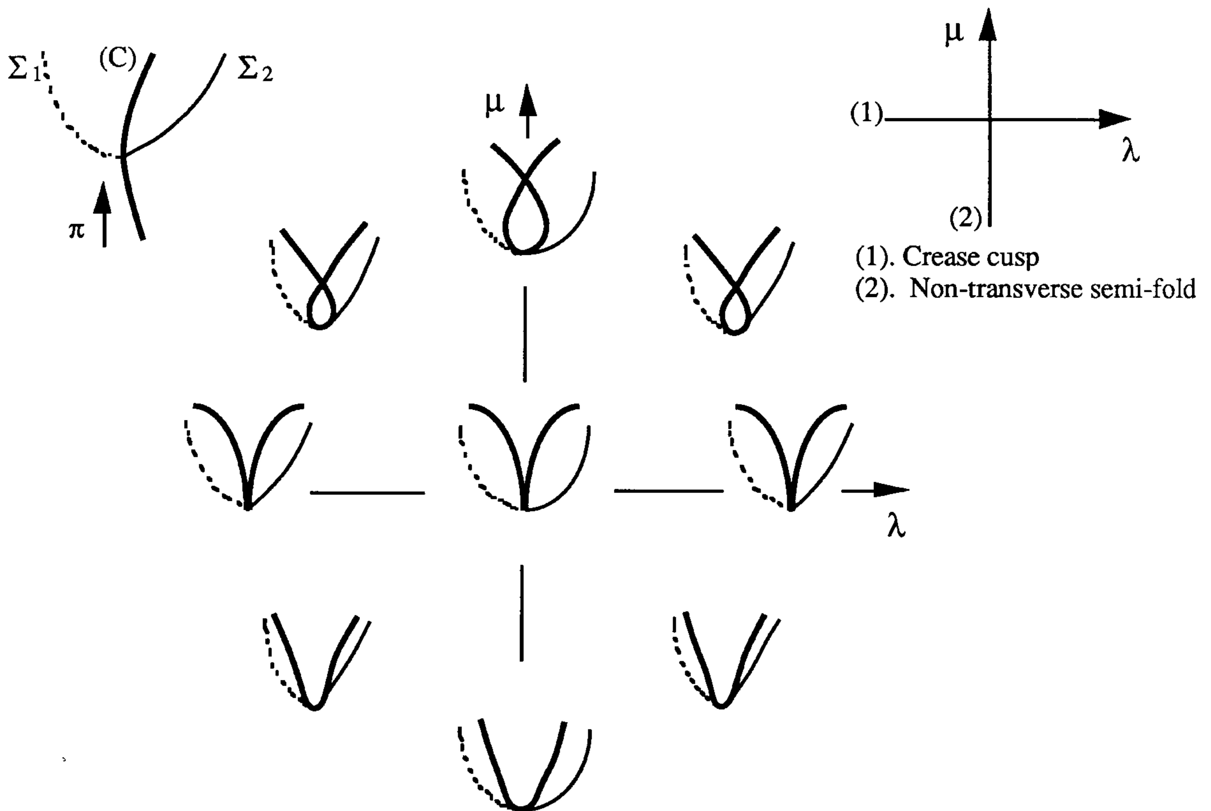
Figure 1.4.14. Non-transverse crease cusp
