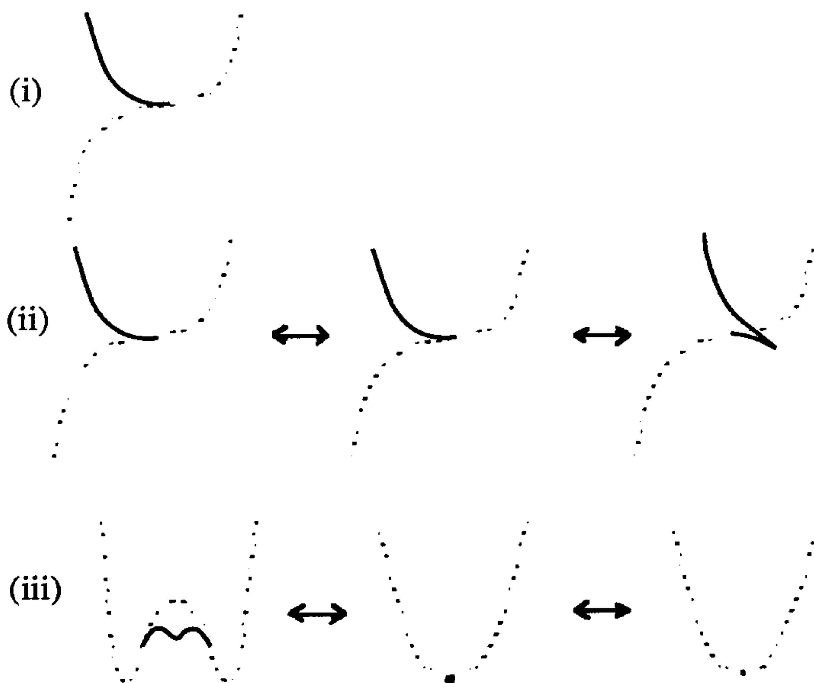
Figure 5.4.2. Transitions on 1-parameter families of RSS^-
