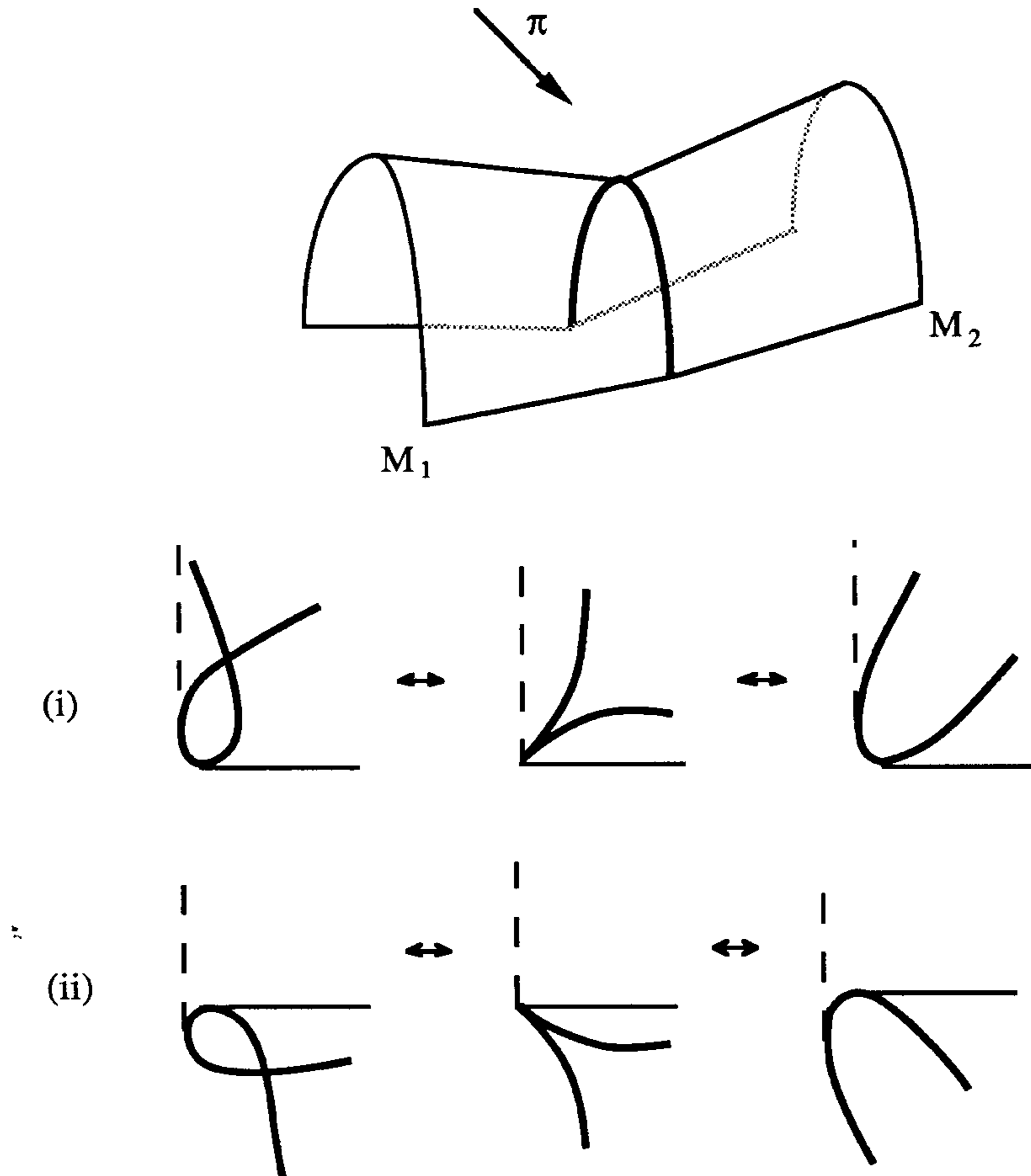
Figure 1.4.7. Crease cusp
