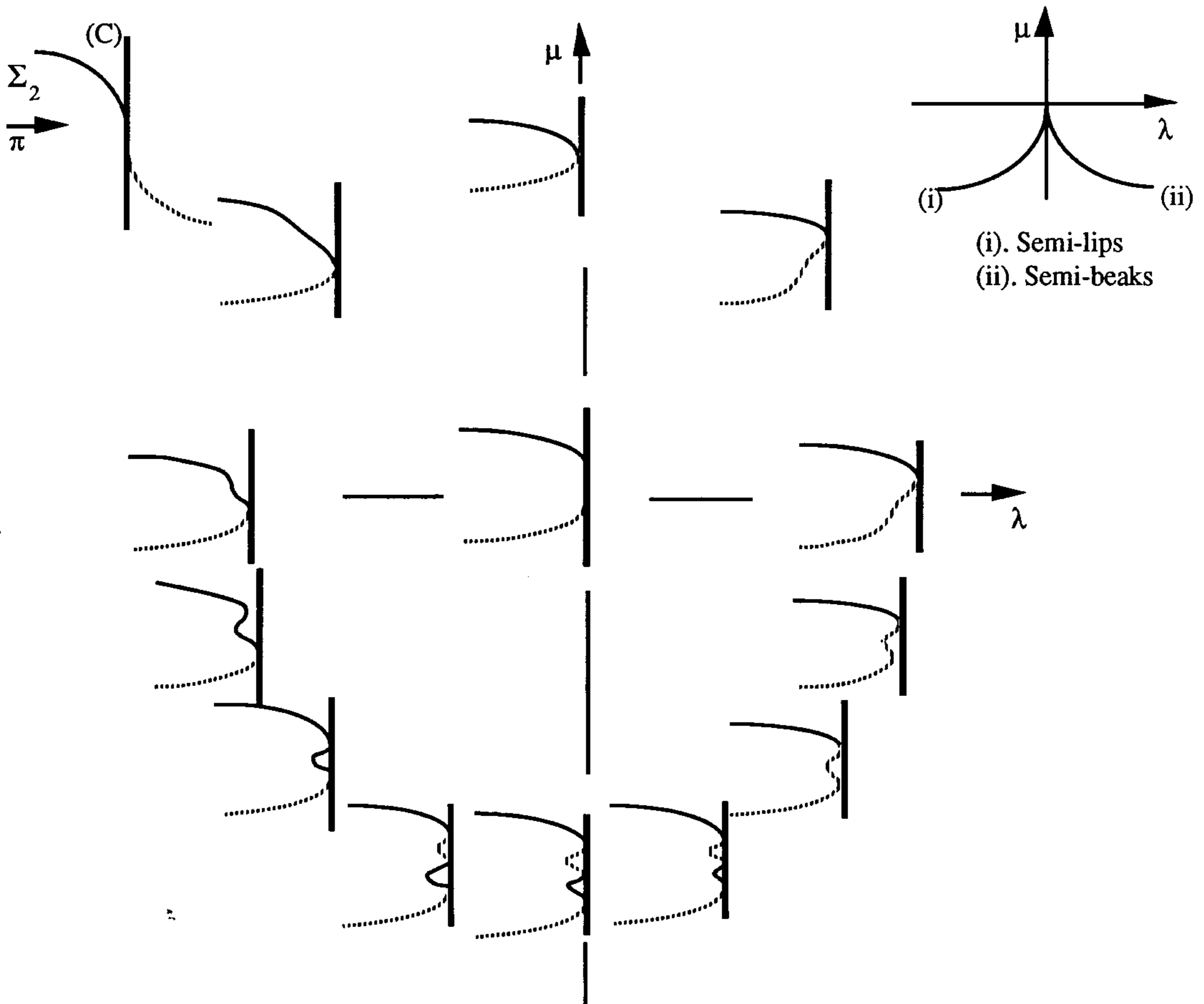
Figure 1.4.3. Semi-goose
