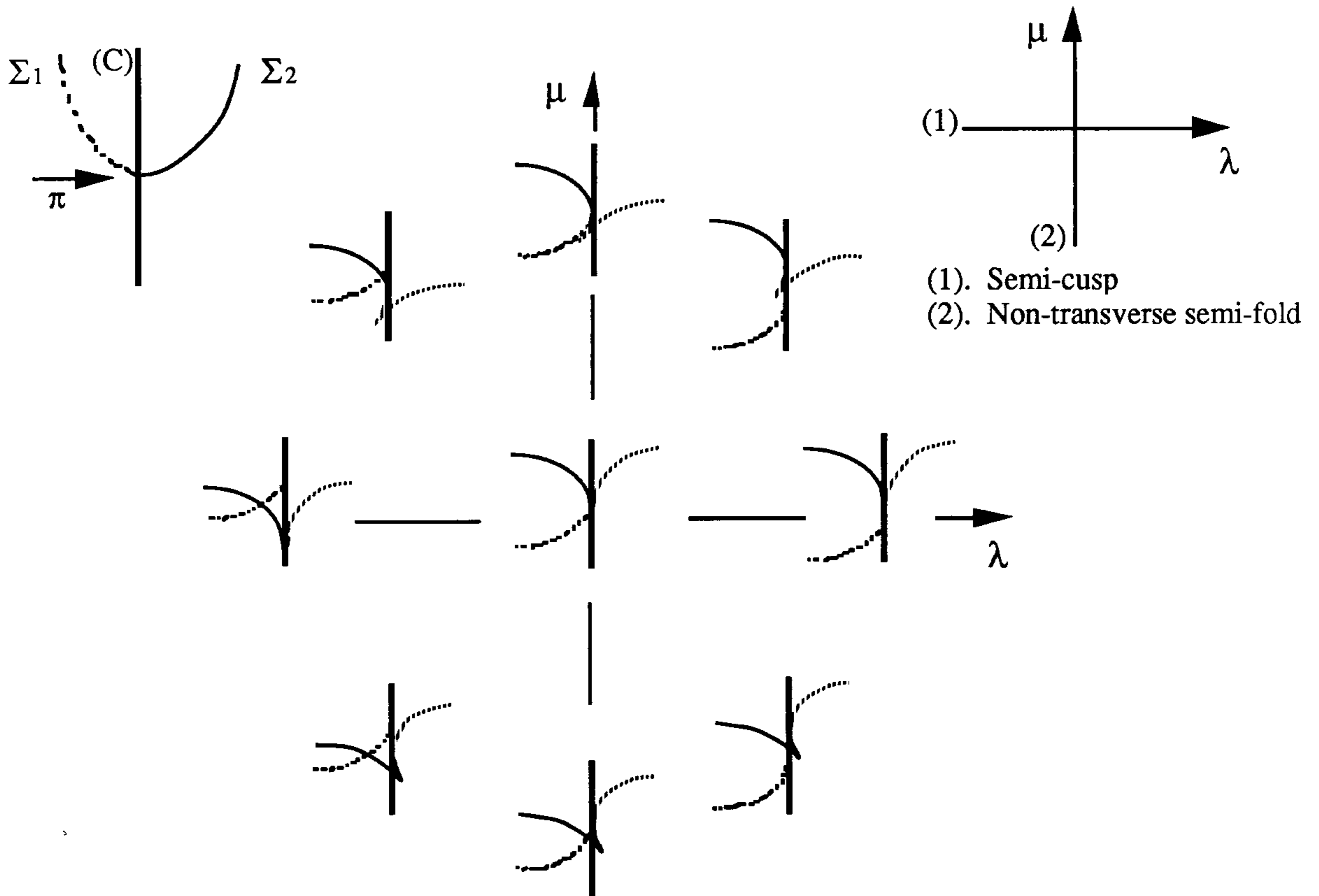
Figure 1.4.13. Non-transverse semi-cusp
